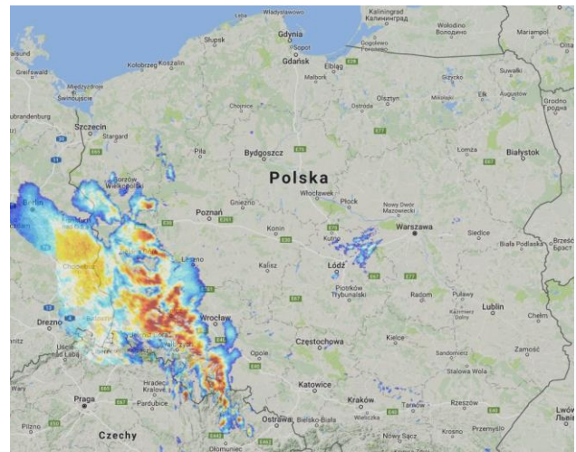
B) CAPPI (1 km) showing reflectivity at the height of 1 km at 16:00 UTC. The line of storm cells formed SLBE moving to Lower Silesia Lowland
