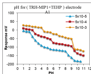
Figure 10. Effect of pH on the tramadol hydrochloride ((TRH-MIP2+DOP (A1)) electrodes at concentrations 5 \times 10^{-3} , 5 \times 10^{-4} and 5 \times 10^{-5}
