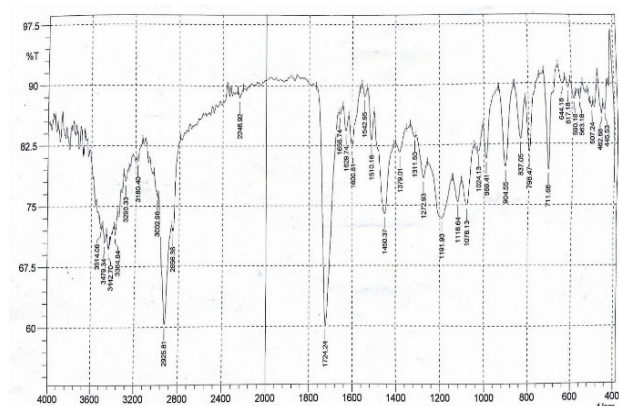
Figure 8. FTIR of TRH-MIP (2-HEMA) after the removal of TRH
