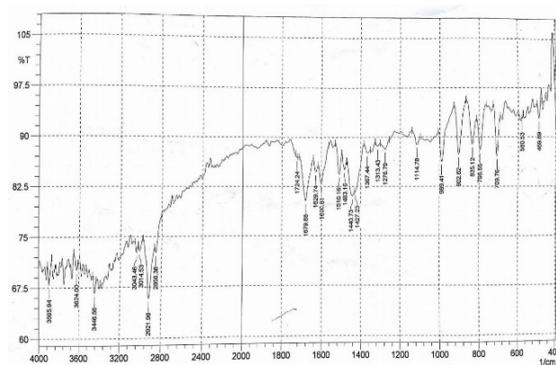
Figure 6. FTIR of TRH-MIP (AA) after the removal of TRH
