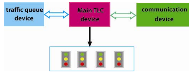
Fig. 2. Block diagram of the developed SOA based ITLCS
