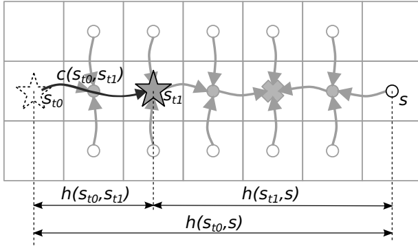
Fig. 3. If the agent (star) moves from s_{t0} to s_{t1} , then the h value of node s will change. For the s node, the previous h value was h(s_{t0}, s) ; however, following the agent's transition, a new h value should be h(s_{t1}, s) . Assuming that for the heuristic function the triangle inequality h(s_{t0}, s_{t1}) + h(s_{t1}, s) \geq h(s_{t0}, s) holds, the worst case of overestimation of the h value for node s , i.e., h(s_{t0}, s) - h(s_{t1}, s) , will be equal to h(s_{t0}, s_{t1}) , though, in general, the traveled path cost c(s_{t0}, s_{t1}) \geq h(s_{t0}, s_{t1}) . If, in the next search episode, the old h value is used for open-list prioritizing, the s node may be removed from the top of the open list too late. White inner shape: open nodes, gray inner shape: closed nodes.
