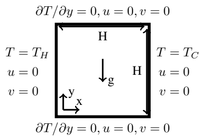
Fig. 10. Configuration of the two dimensional cavity.
