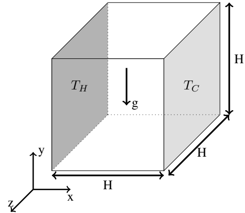
Fig. 13. Configuration of the three dimensional cavity.
