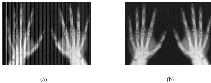
Fig. 7. Restoration arising from the LS solution and the Moore-Penrose inverse: LS solution (a), Moore-Penrose inverse solution (b).
