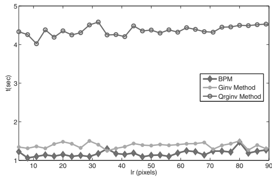
Fig. 1. CPU time for computing the MP inverse of the random matrix H versus l_r ( l_c = 30 ).
