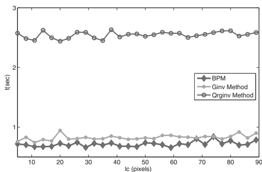
Fig. 4. CPU time for removing a blur caused by the Gaussian function and noise versus l_c ( l_r = 35 ).
