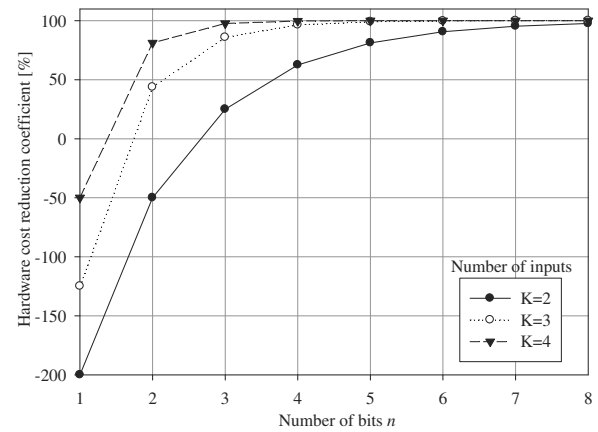
Fig. 7. Hardware cost reduction coefficient vs. the number of bits of input and output values and the number of inputs for relational fuzzy systems (FATI).
