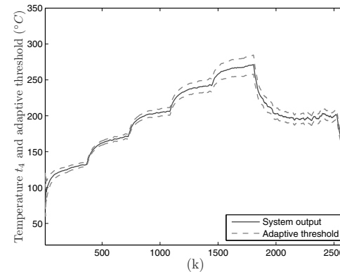
Fig. 18. Temperature t_4 of the furnace and the corresponding adaptive threshold obtained with the GMDH model.
