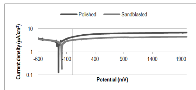
Fig. 3. Polarisation curves of plasma nitrided in 35:65 H 2 :N 2 gaseous mixture 440B steel in 0.9 wt% NaCl solution (unde-aerated, unstirred)
