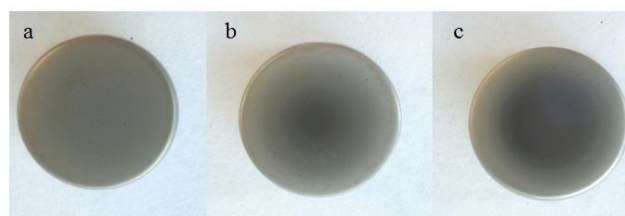
Fig. 7. Plasma nitrided polished specimens; a – 50% H 2 :50% N 2 , b – 35% H 2 :65% N 2 , c – 20% H 2 :80% N 2 ; macro photographs
