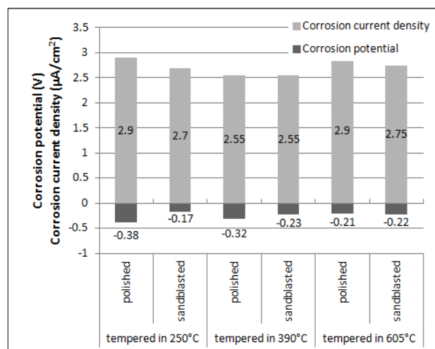
Fig. 4. Conventionally heat treated specimens corrosion potentials and corrosion currents densities
