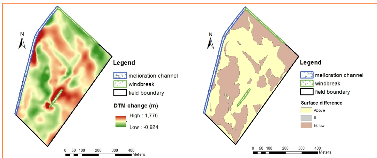
Figure 2 Digital terrain model change map of selected field
