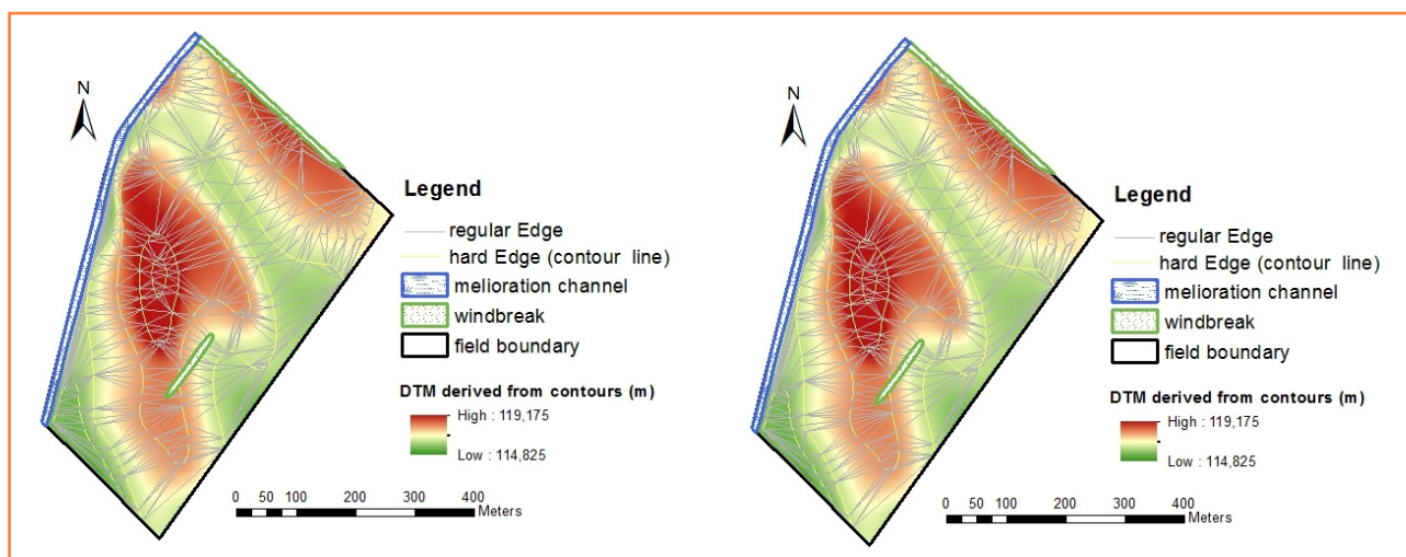
Figure 1 TIN models: left side derived from contours, right side derived from measured points
