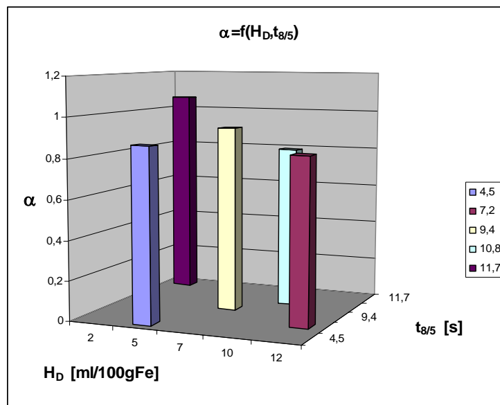
Fig. 3. The influence of the diffusible hydrogen H_D and the cooling time t_{8/5} on resistance to cold cracking indicator \alpha for joints made by MMA and FCAW methods on P460NL1 steel
