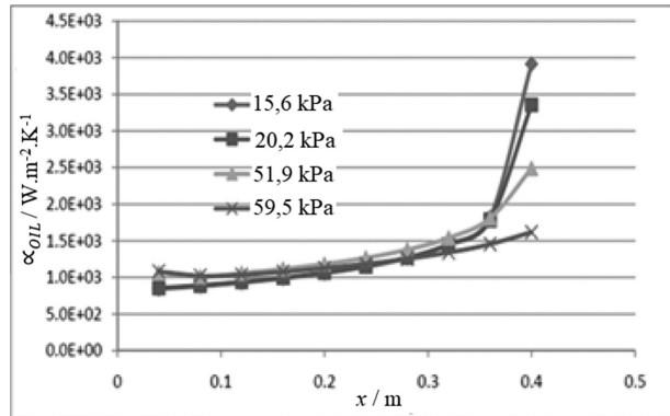
Fig. 4. Heat transfer coefficients \alpha_{OIL} of oil along the vertical tube.
