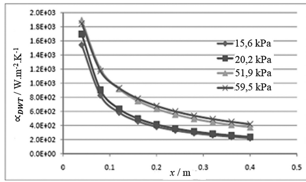
Fig. 3. Heat transfer coefficients \alpha_{DWT} of Dowtherm A along the vertical tube.
