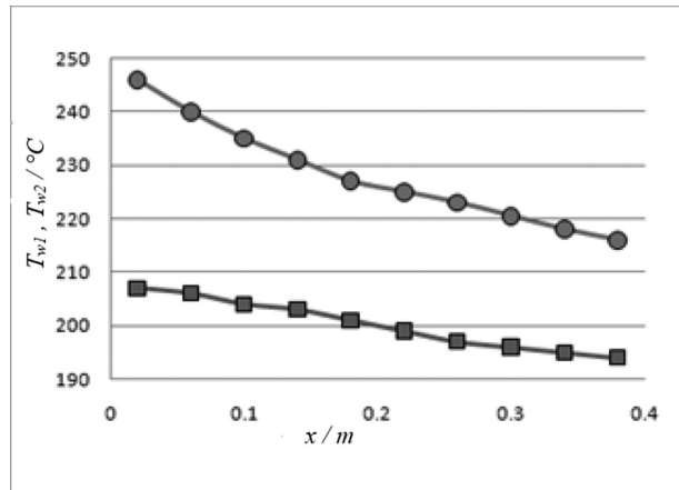
Fig. 5. Variation of the mean wall surface temperatures T_{w1} and T_{w2} along the tube axis direction for distillation pressure 20.2 kPa.
