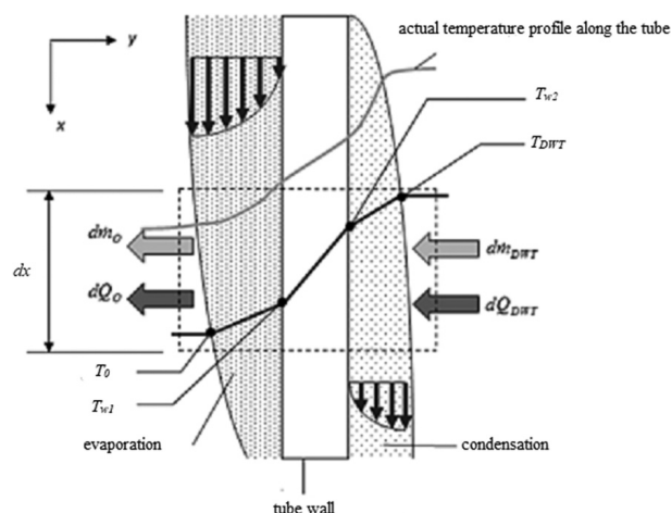
Fig. 2. Temperature profile along the vertical tube.
