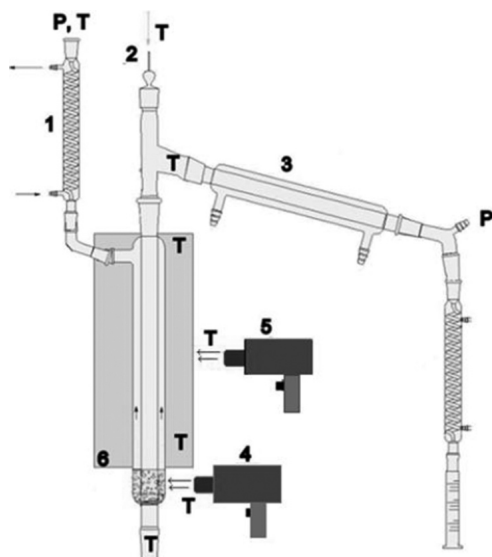
Fig. 1. Experimental equipment description.
